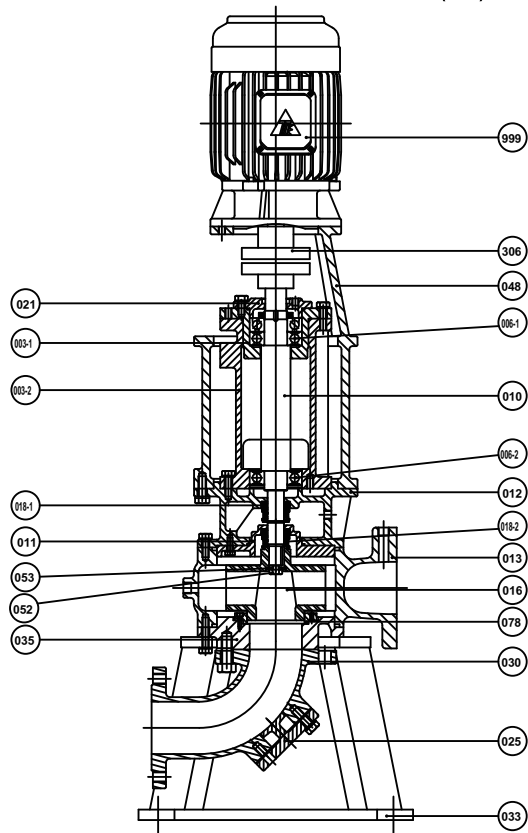
CVD乾井立式聯軸不堵塞污物(泥)泵
